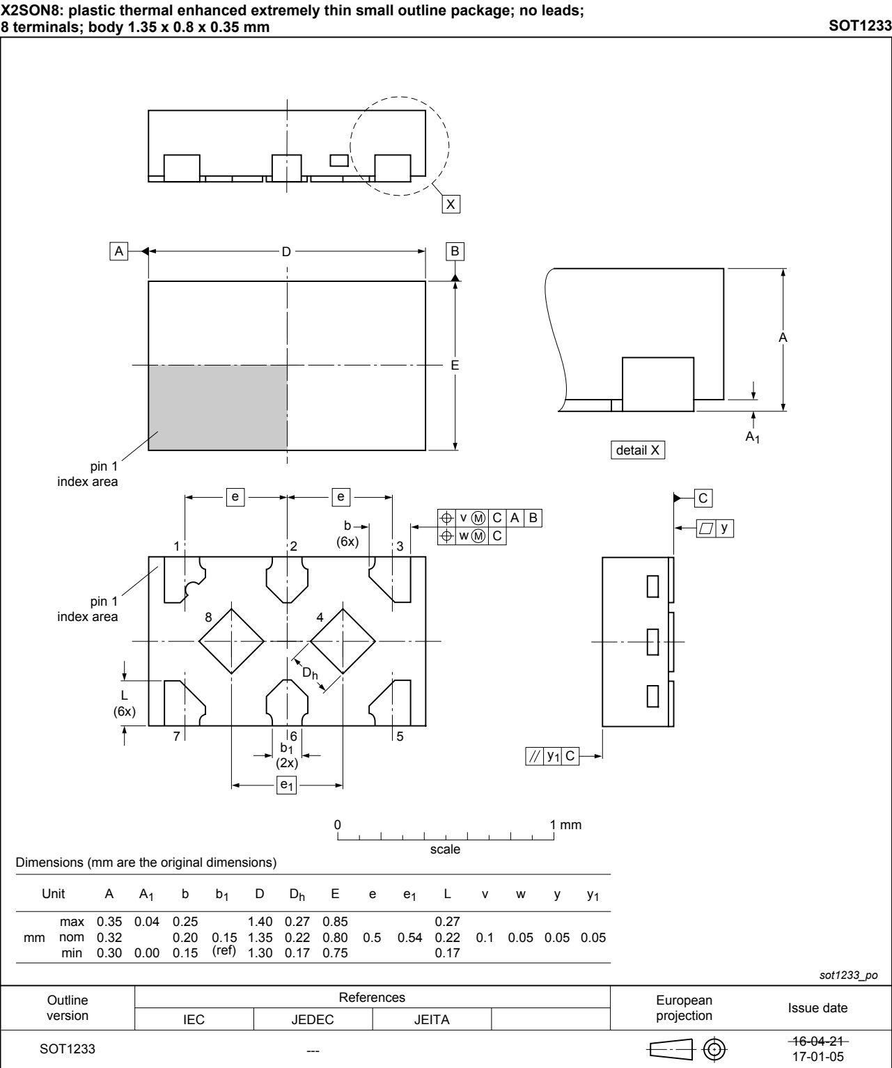
Figure 19. Package outline SOT1233 (X2SON8)
